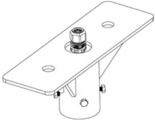
2 3/8 inch Tenon Mount KIT, CLIR, PTM Pole 2 3/8 inch
